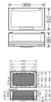
S-DP8/DP32 Dimensions
