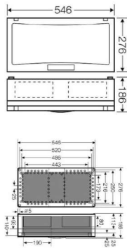
S-DP4 Dimensions
